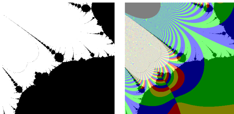
FIG. 3.1: LEFT: A_\phi AT THE EDGE OF THE MAIN CARDIOID; RIGHT: SUPERIMPOSED QUADRANT PLOT OF \zeta^{\circ 2}
